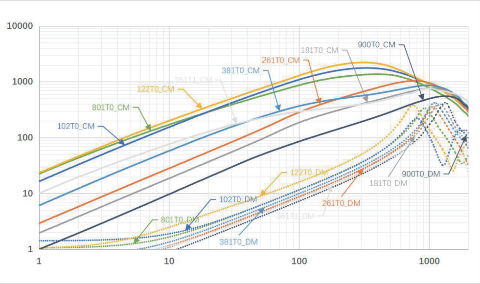
5 Impedance VS. Frequency
