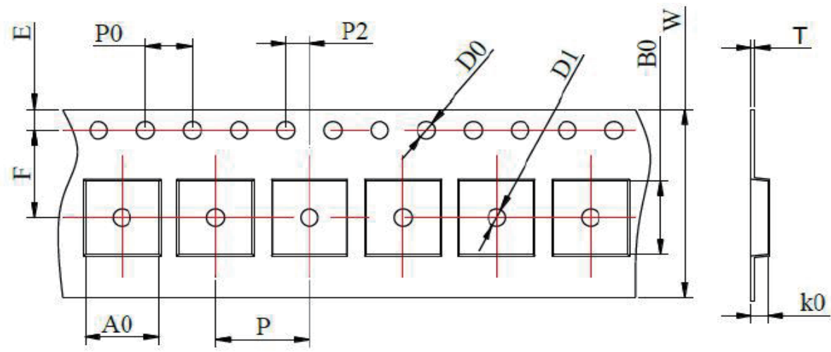
(1) Tape Packaging Dimensions (Unit: mm)
