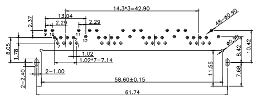
RECOMMENDED PCB LAYOUT (TOP VIEW) (ALL TOLERANCES ARE ±0.05)
