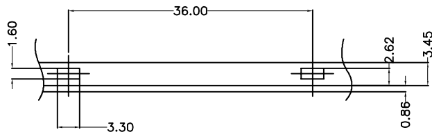
RECOMMENDED BRACKET CUTOUT
