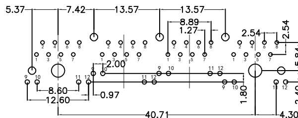
RECOMMENDED PCB LAYOUT VIEWED FROM COMPONENT SIDE
