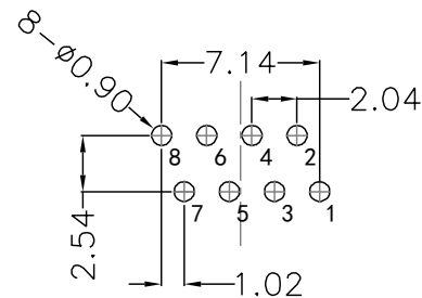
RECOMMENDED PCB LAYOUT VIEWED FROM COMPONENT SIDE
