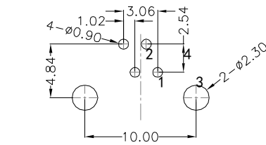
RECOMMENDED PCB LAYOUT VIEWED FROM COMPONENT SIDE
