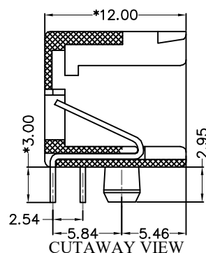
CUTAWAY VIEW
