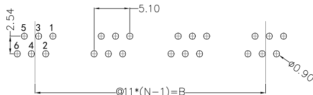
RECOMMENDED PCB LAYOUT VIEWED FROM COMPONENT SIDE
