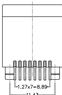
BACK VIEW
