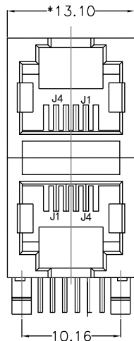
FRONT VIEW
