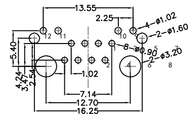
RECOMMENDED PCB LAYOUT VIEWED FROM COMPONENT SIDE
