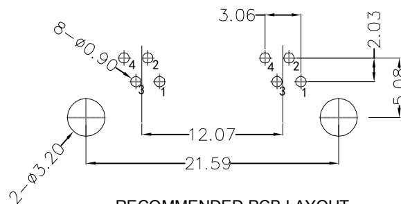
RECOMMENDED PCB LAYOUT VIEWED FROM COMPONENT SIDE
