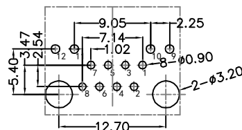
RECOMMENDED PCB LAYOUT VIEWED FROM COMPONENT SIDE
