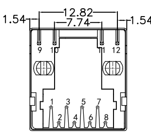
BACK VIEW
