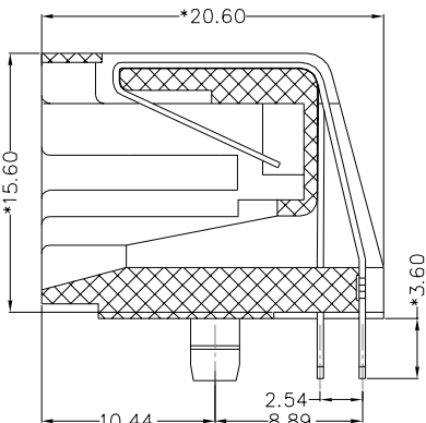
CUTAWAY VIEW
