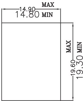
Single Panel-Latch Clearance Panel Thickness 1.60mm
