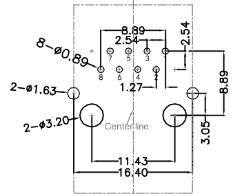
RECOMMENDED PCB LAYOUT VIEWED FROM COMPONENT SIDE
