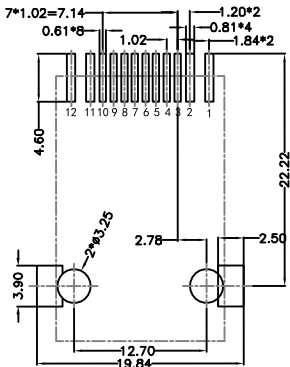
RECOMMENDED PCB LAYOUT VIEWED FROM COMPONENT SIDE
