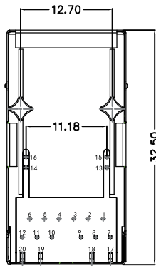
BOTTOM VIEW
