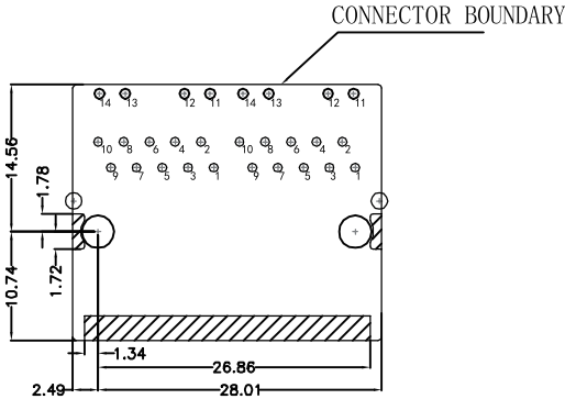
PLUG-IN SIDE
