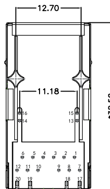
BOTTOM VIEW
