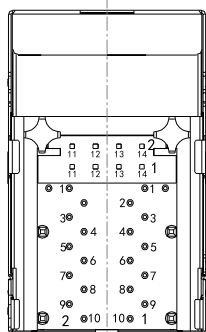
BOTTOM VIEW
