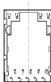
BACK VIEW
