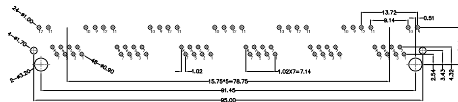
RECOMMENDED PCB LAYOUT VIEWED FROM COMPONENT SIDE
