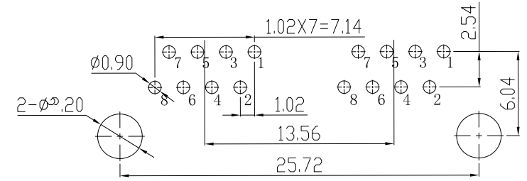
PC Board Layout T=1.6mm
