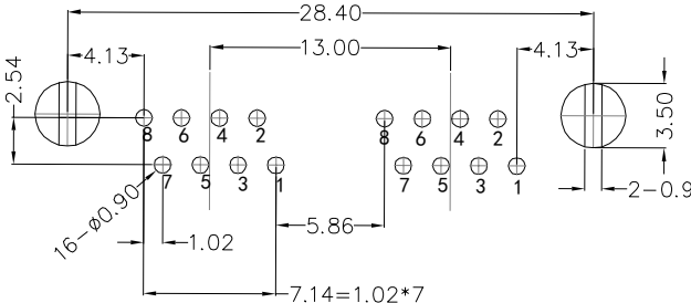
RECOMMENDED PCB LAYOUT VIEWED FROM COMPONENT SIDE
