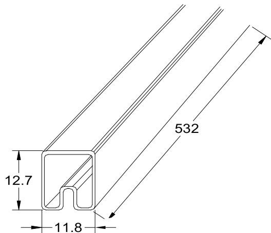
Tube: 532*11.8*12.7mm
