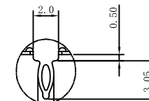
DETAIL B SCALE 5:1
