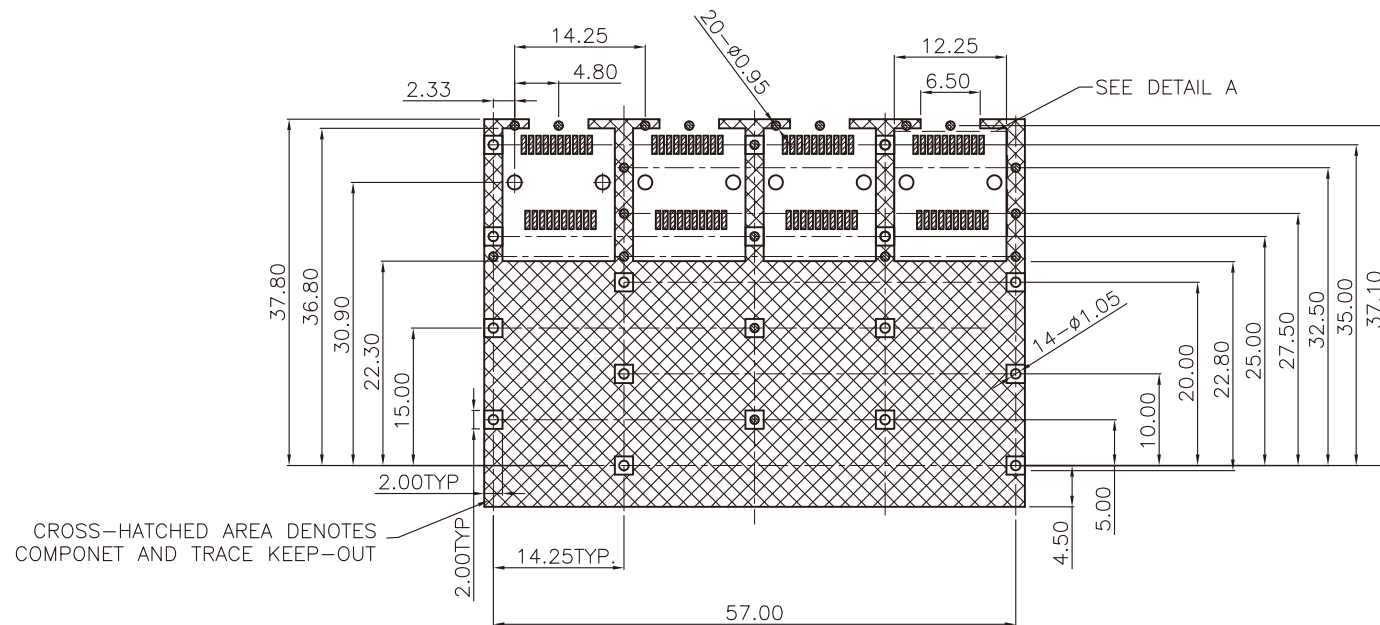
RECOMMENDED PCB LAYOUT (COMPONENT SIDE)
