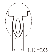
DETAIL B SCALE 5:1
