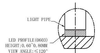
DETAIL F SCALE 4:1
