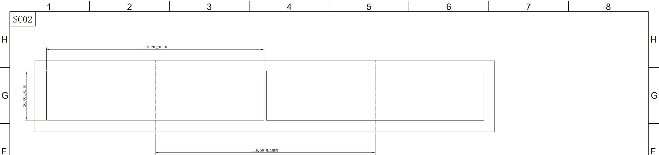
BEZEL CUT-OUT CENTER SPACING DETAIL BZZEL THICKNESS:0.8-2.6
