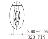
DETAIL A SCALE 10:1
