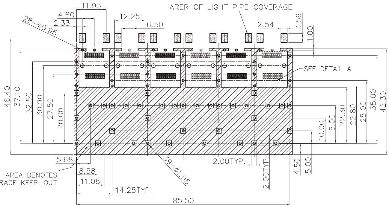
RECOMMENDED PCB LAYOUT (COMPONENT SIDE)
