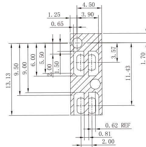
KEEPOUT ZONE DETAIL SCALE 5:1
