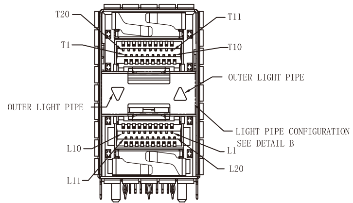
DETAIL A
