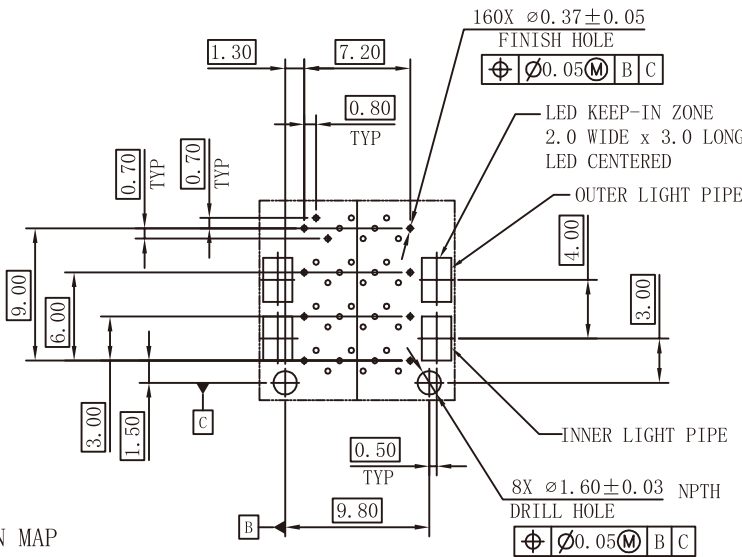
DETAIL C SCALE 2:1
