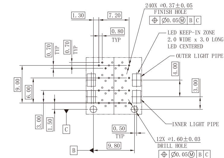
PIN MAP
