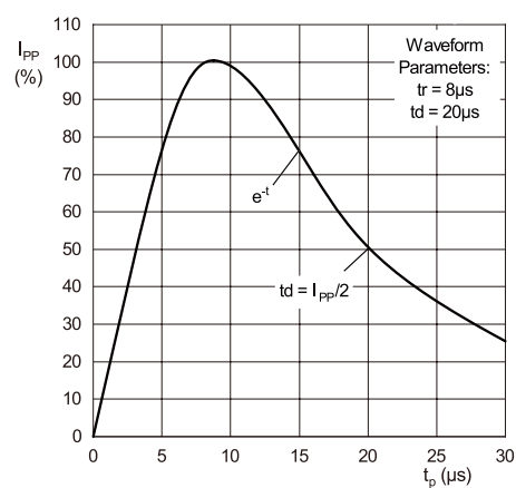
Figure 3 Pulse waveform
