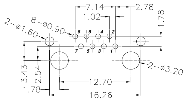
RECOMMENDED PCB LAYOUT VIEWED FROM COMPONENT SIDE
