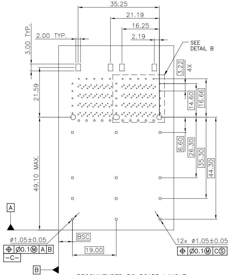
RECOMMENDED PC BOARD LAYOUT COMPONENT SIDE OF BOARD (PCB TOLERANCE \pm 0.05 )
