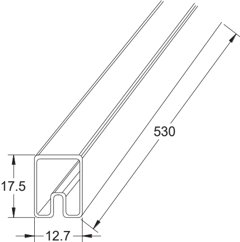
Tube: 530*17.5*12.7mm
