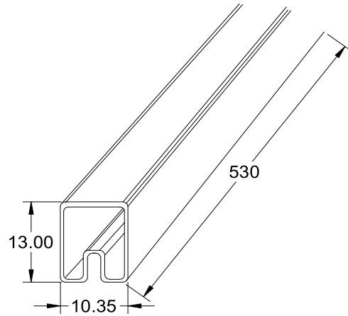
Tube: 535*13.0*10.35mm
